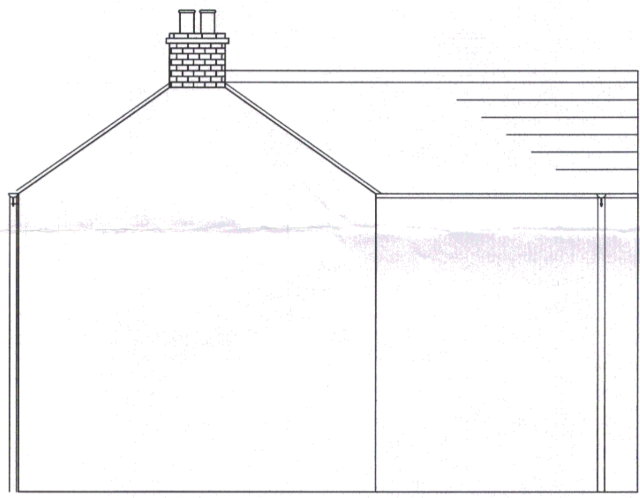
S ELEVATION SOUTH 1:50
